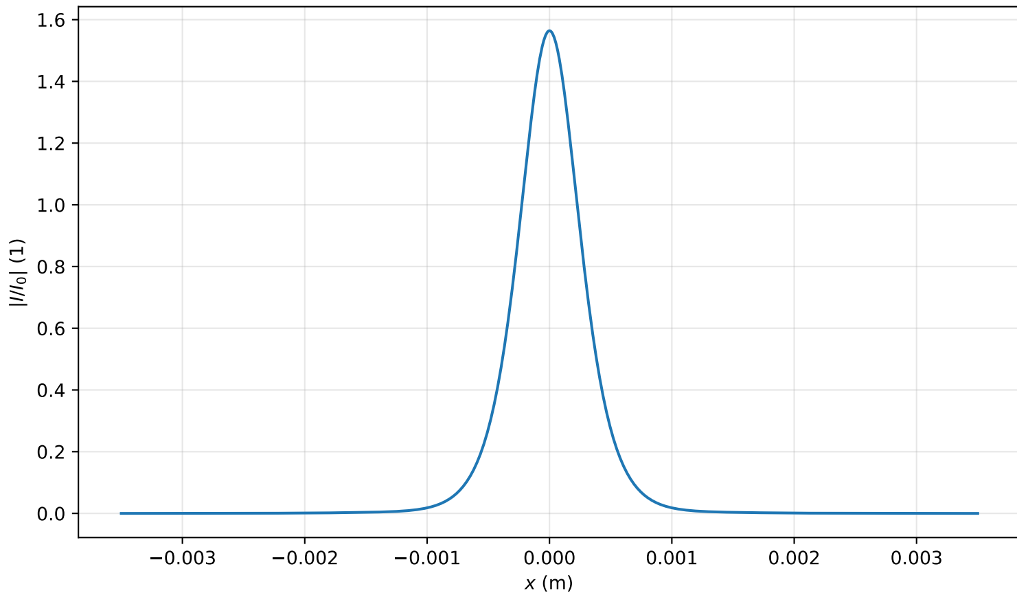
Intensity profile I(x, y = 0, z = 3.025m)/I_0 , P_{in}=0.9P_{cr} , artificial time
